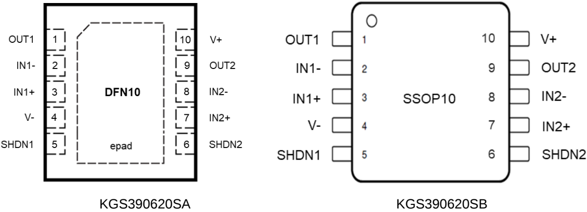
Figure 4 KGS390620SA/B Pinouts
