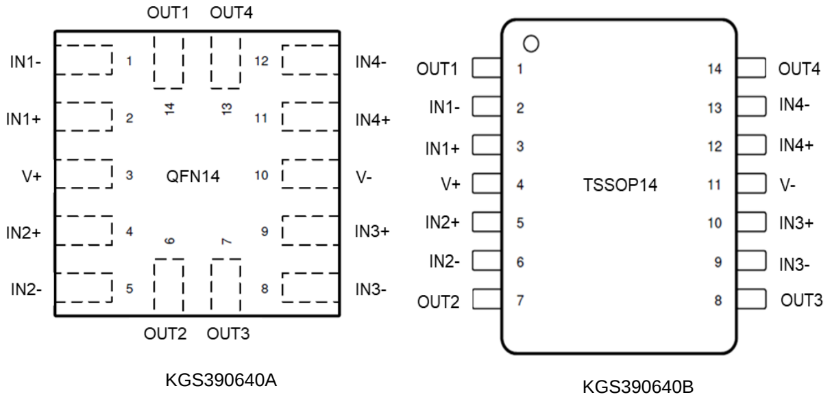
Figure 5 KGS390640A/B Pinouts
