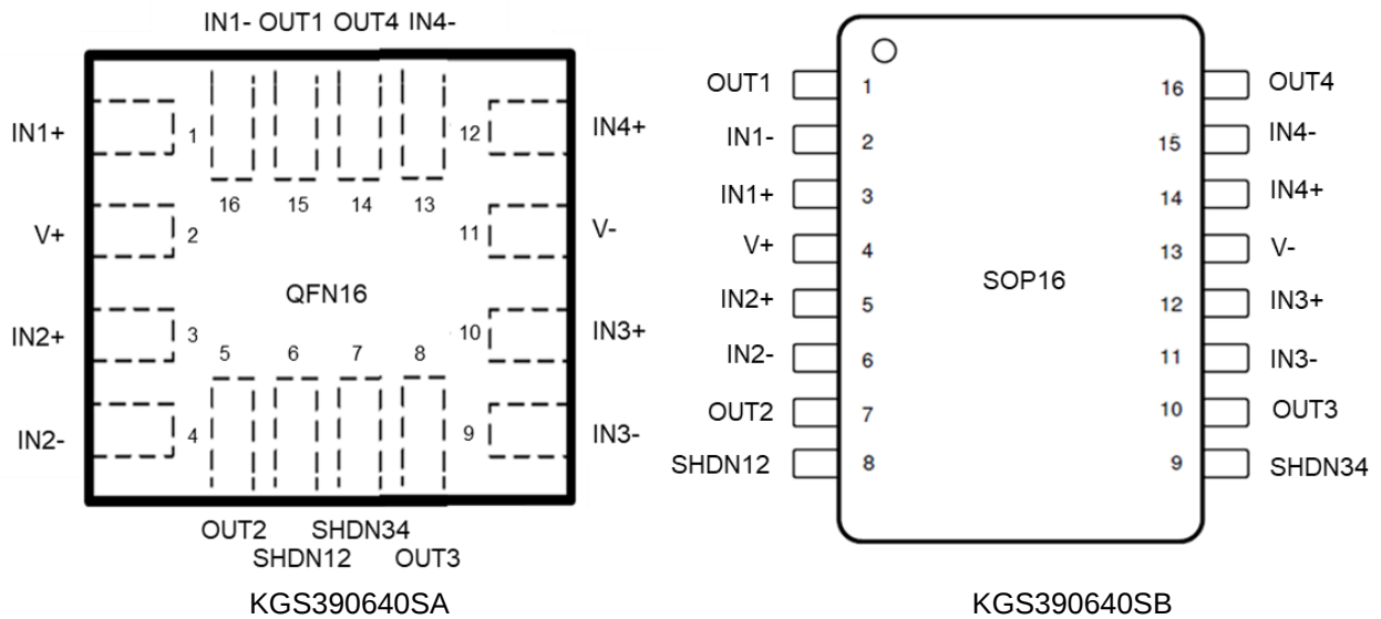
Figure 6 KGS390640SA/B Pinouts
